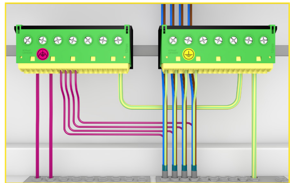
Mark functional potential bonding for better orientation. Connect main grounding busbar to PE as usual, connect busbar FPA and busbar PE with \geq 4 \text{ mm}^2 cross-section.
