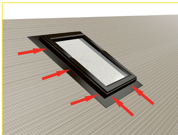
Fig.45: Connection to roof window installation under roofing frame up to window
