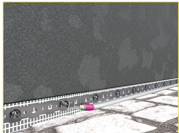
Fig.34: Connection of the grounding conductor with RKS16
