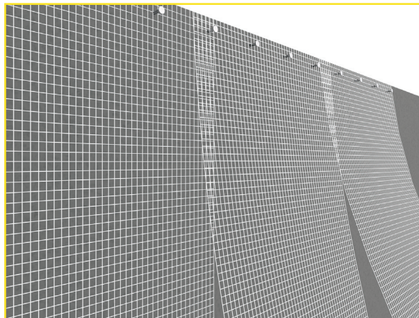
Fig.8: Provisional fixture of the fabric sheets
