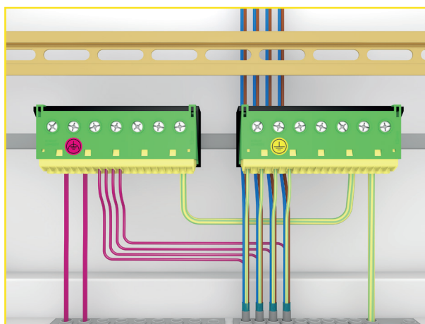
Fig. B1: Connection left of the functional equipotential bonding conductor in the lower main distributor of the power supply with the separately marked functional equipotential bonding rail.
