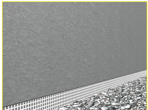
Fig.32: Socket area left free by about 5 cm
