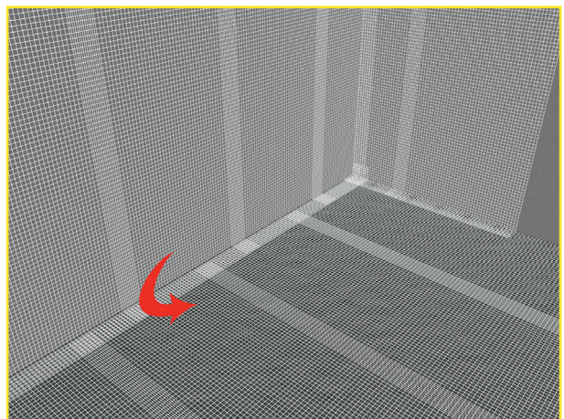
Fig.22: Overlap from wall to floor.
