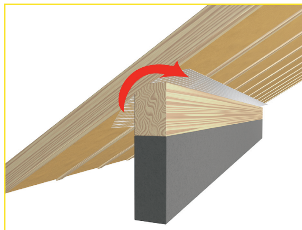
Fig.41: Option – Transition from facade to roof, outside to inside, between purlin and rafters.
