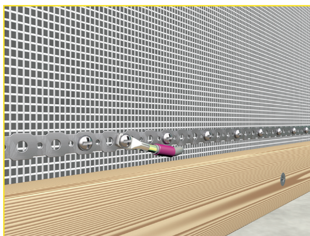
Fig.10: Attaching the stainless steel ground strap EEB with stainless steel screws – grounding with RKS
