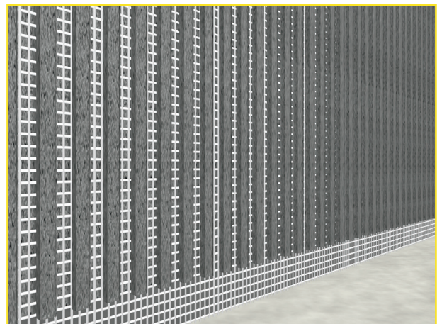
Fig.2: Embedding compound, notched trowel, and fabric incorporation
