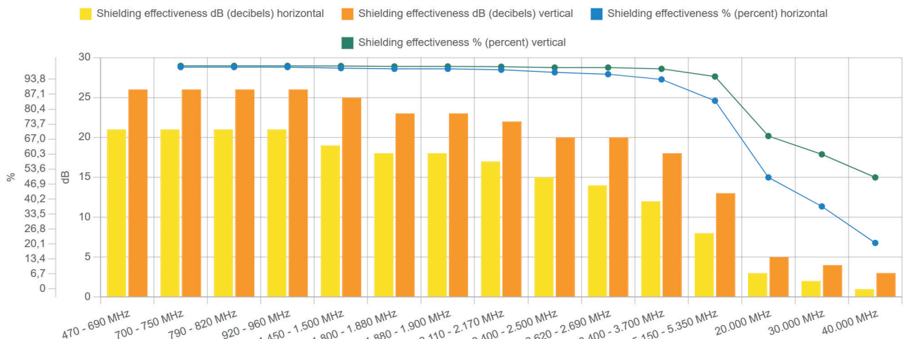
Shielding effectiveness - Antiwave OC white - stretched - 470 MHz to 40.000 MHz (40 GHz)
