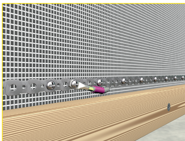
Fig. 3: Attaching the stainless steel grounding strap EEB with stainless steel screws. Pink/pink marking. Grounding with RKS.
