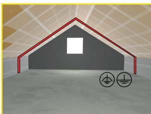
Fig. 16a: Grounding sloping roof with EEB
