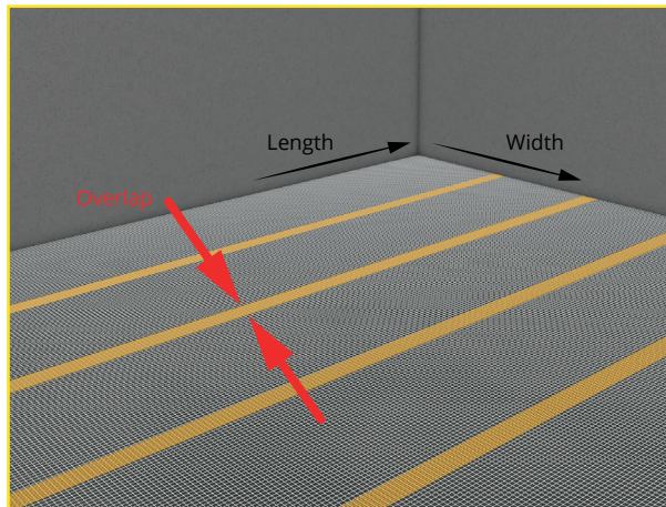
Fig. 7: Length and width of the surface / overlap
