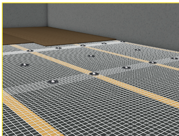
Fig. 9: Fastening the shielding sheets / overlapping areas
