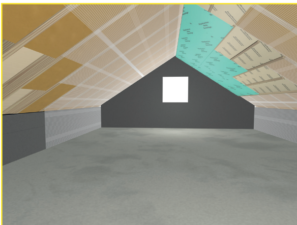
Fig. 16: Laying on rafters or between two layers of panels. Earthing diagram see Fig. 16a
